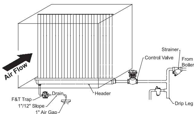
Figure 80-1. HumidiPack
