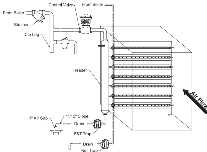
Figure 80-2. HumidiPackPlus
