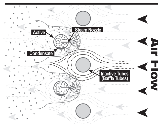
Figure 81-4. Mixing of Air and Steam (HumidiPack shown)
